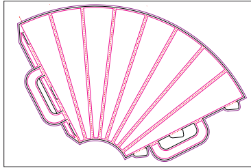
Product No. YD-114 Name: Megaphone Sheet size: 20.5 x 14.33 Size Specs: 11 inches long
