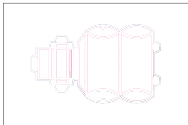
Product No.YD-010 Name: Thumb Drive Mailer Sheet size: 18 x 12 (1-up) or 20.5 x 14.33 (2-up) Size Specs: 5 x 3 x 1.875 approx.
