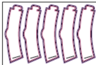
Product No. YD-034 Name: Cup Sleeve 5-Up Sheet size: 18" x 12" without tape Size Specs: 2.25" x 10"
