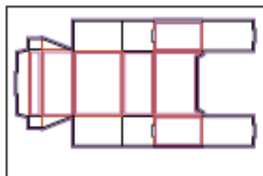
Product No. YD-039 Name: Index Box - Small 1-Up Sheet size: 17" x 11" Size Specs: 4.13" x 3.18" x 2"
