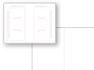
Product No. CP-075 A combined item of YD-074 and YD-076 Name: Folder with Affixable Print Pockets Contains: 18 x 12 flat sheet folder, and two 17 x 11 - Pre-Taped L&R Pockets; Assembled product is a 9 x 12 folder w/2-4 Pockets; 12pt to 18pt body /12pt to 14pt Pockets
