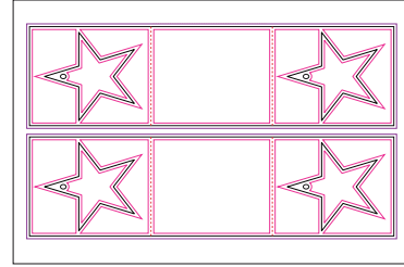
Product No. YD-116 Name: 2-Up Star Ornament Card Sheet size: 12 x 18 Size Specs: 4.5 x 5.5 folded 6 panel
