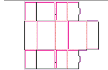
Product No. YD-047 Name: General Purpose Box - Small 1-Up Sheet size: 19" x 13" " Size Specs: 6" x 3.875 x 2.5"
