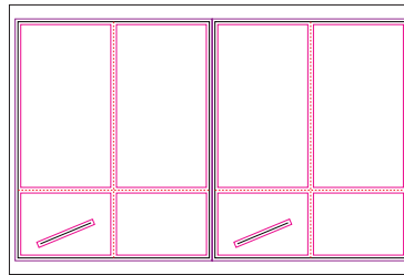
Product No. YD-058 Name: Mini Pocket Folder 2-Up Sheet size: 18" x 12" Size Specs: 4.25" x 7.5" x with 2- 3" pockets
