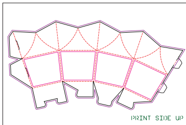
Product No. YD-096 Name: 1 CB Flower Top Box 1-Up Sheet size: 18 x 12 Size Specs: 5.5 x 4.25
