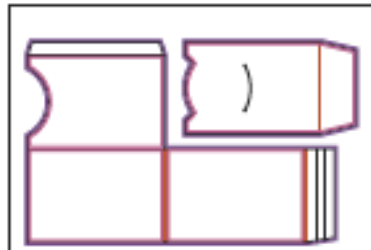
Product No. CP-033 Name: Slide Out CD Sleeve Sheet size: 18" x 12" without tape Size Specs: 5.25" x 8"
