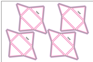
Product No. YD-048 Name: Gift Card Holder 4-Up Sheet size: 18" x 12" Size Specs: 3.5" x 2.25"
