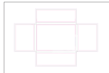
Product No.YD-009 Name: Photo Box Mailer Sheet size: 18 x 12 Size Specs: 4.25 x 6.375 x 0.25
