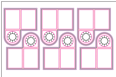
Product No. YD-072 Name: 4 Page Bottle Necker 6-Up Sheet size: 18 x 12 Size Specs: 2.5 x 3.31 (5.68)
