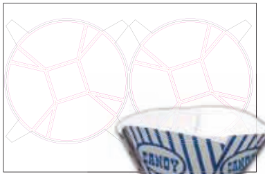
Product No.YD-021 Name: Sm.Popcorn Treat Bowl 2-up Sheet size: 18 x 12 Size Specs: 3.25 deep, 2 x 2 base by 6 open top
