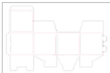
Product No.YD-001 Name: Cube Box 4 x 4 Sheet size: 18 x 12 Size Specs: 4x4 with tabbed top lid
