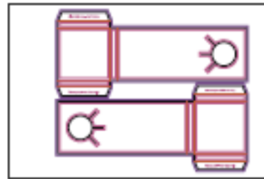
Product No. YD-037 Name: Pocket Door Hanger 2-Up Sheet size: 18" x 12" with tape Size Specs: 3.68" x 9", 3.63" x 3.63" x .5"
