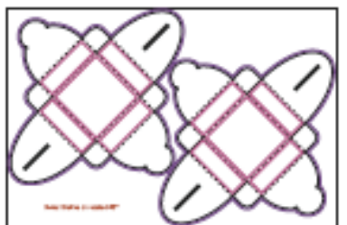
Product No. YD-041 Name: Fold Up Box 2-Up Sheet size: 18" x 12" Size Specs: 3.75" x 3.75" x 1.25"
