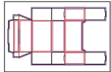
Product No. YD-038 Name: Index Box - Full Size 1-Up Sheet size: 17" x 11" Size Specs: 5.19" x 3.18" x 2"
