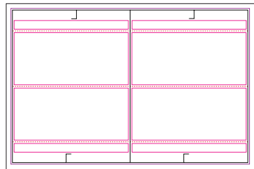
Product No. YD-081 Name: Landscape Tent Card 2-Up Sheet size: 18 x 12 Size Specs: 4 x 8.5 x 1.5
