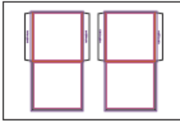
Product No. YD-025 Name: CD Sleeve 2-Up Sheet size: 18" x 12" without tape Size Specs: 5.25" x 5.25"
