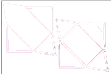
Product No.YD-013 Name: Invite Mailer 2-Up Sheet size: 18" x 12" Size Specs: 4" x 6"
