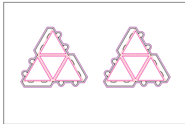
Product No. YD-069 Name: Pyramid Box 2-Up Sheet size: 18 x 12 Size Specs: 3.05 x 3.05 x 2.39
